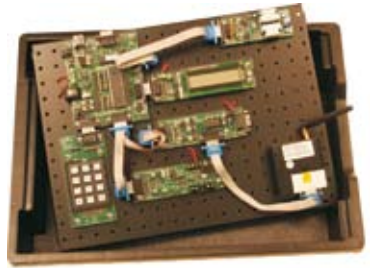
Fig 24 - A completed E-blocks system with tray
